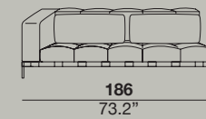
19_3 seats (1 mechanism) left arm 20_3 seats sofa (1 mechanism) right arm
