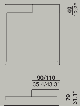
LOW HEADBOARD RIGHT
